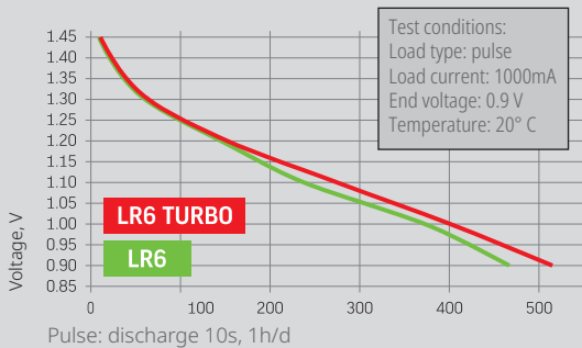
Discharge comparison of LR6 TURBO and LR6
